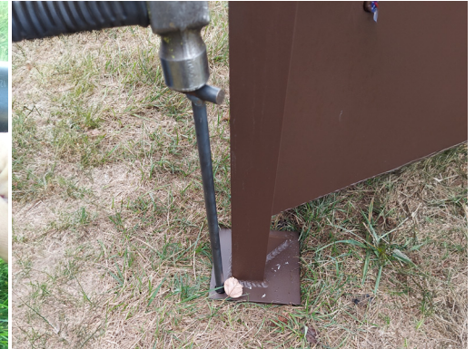
STEP 18 Install 2 ground stakes in hopper base. Always install feeder level so corn empties completely keeping feeder clean...pipe can go up or down hill but keep feeder level
